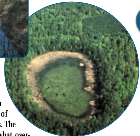
Wetlands range from permanent ponds (above), to short-lived roadside ditches, to seasonal wetlands like Carolina bays (below) that may hold water for many months in some years and remain relatively dry in others.
